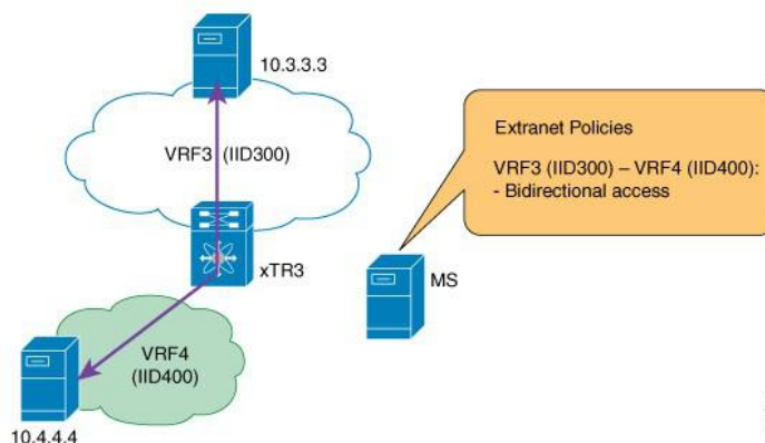
Figure 25 : Local LISP Extranets
