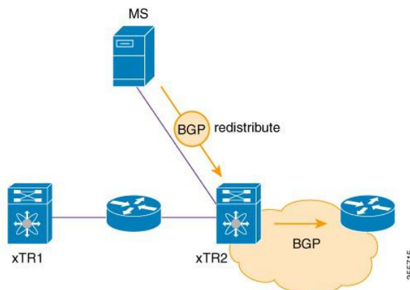
Figure 28 : Redistribute RIB Routes into Map-cache Topology
