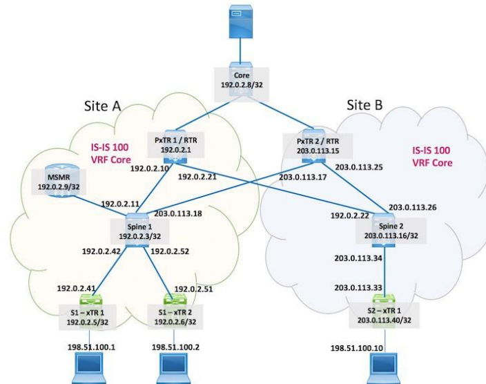
Figure 19: Sample topology—LISP Support for Disjointed RLOC Domains
