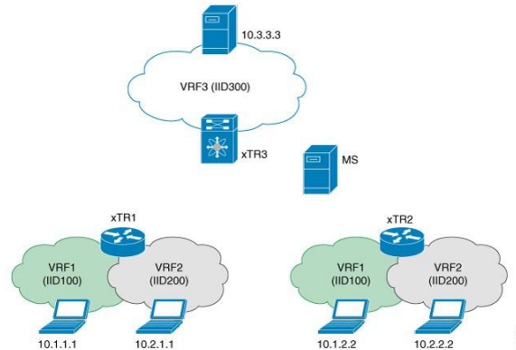
Figure 23 : LISP Extranet Topology
