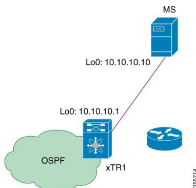
Figure 27 : Redistribute RIB Routes into Database Topology
