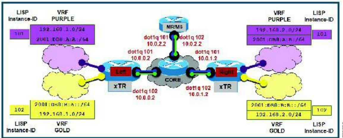
Figure 17 : Simple LISP Site with One IPv4 RLOC and One IPv4 EID
