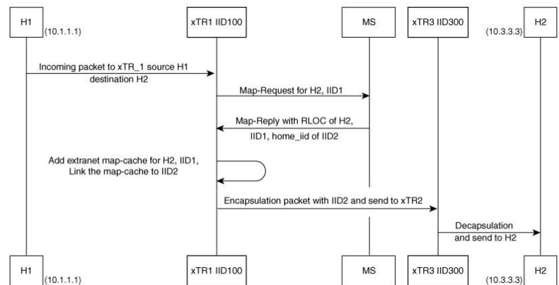
Figure 21 : Packet Flow in LISP VRF Leaking
