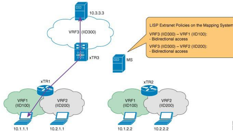
Figure 20 : Inspur INOS LISP Extranets Topology
