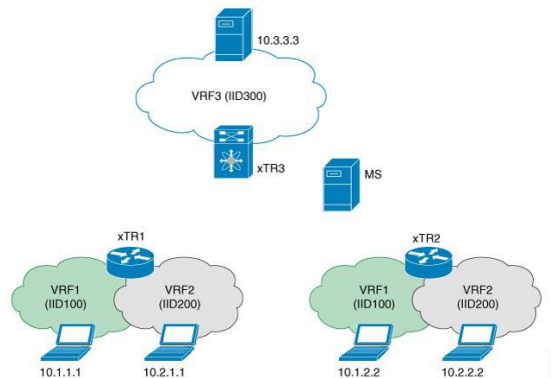
Figure 24 : LISP Extranets Topology
